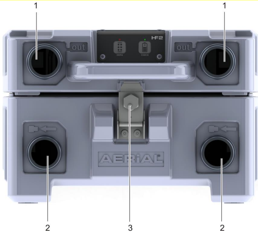
Fig. 1: HEPA Filter series HF2 - overview
